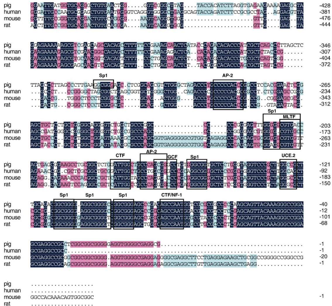
Fig. 2. Sequence alignment of the regulatory regions of the porcine, mouse, rat and human TGFBR1 gene. A 500-bp-long homologous nucleotide sequences of the 5'-flanking regions of the porcine, mouse, rat and human are aligned. Important putative promoter elements are indicated by boxes including CCAAT-box binding transcription factor (CTF), stimulatory protein 1 (Sp1), upstream control element (UCE.2), GC-binding factor (GCF), activating enhancer binding protein 2 (AP-2), and major late transcription factor (MLTF). These putative transcription factors are also shown proximal to the transcription initiation site.
